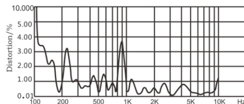
Distortion (THD < 5% 1W, 1m, 100Hz-10kHz)
