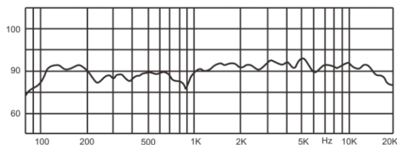
Frequency Response (dB SPL, 1m, 1m)
