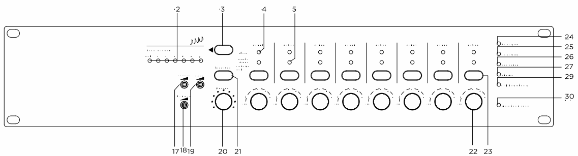
PAVA7000E (8-Zone Expansion Amplifier with Main/Backup Switching Function)
