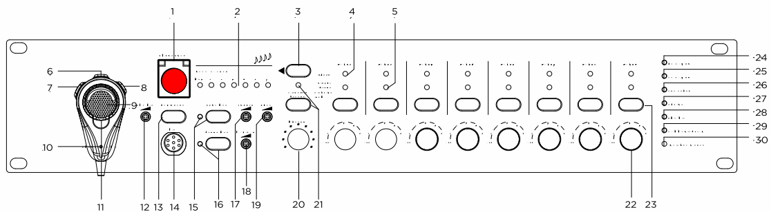
PAVA7000 (8-Zone Amplifier Host with Main/Backup Switching Function)
