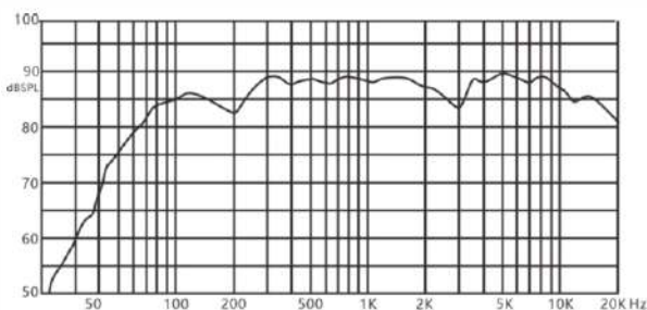
CNS8063 Frequency Response (dB SPL, 1W, 1m)
