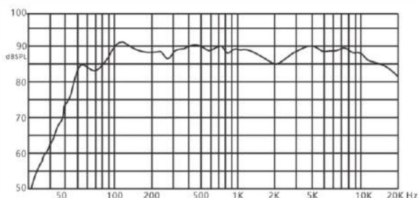
CNS8064 Frequency Response (dB SPL, 1W, 1m)
