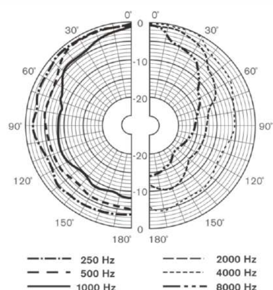
CNS8064 Horizontal Directivity Pattern
