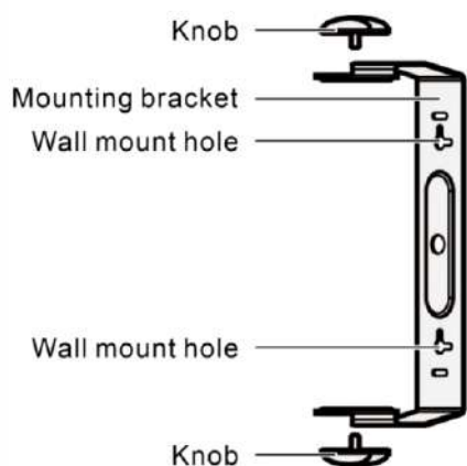
U-shape bracket
