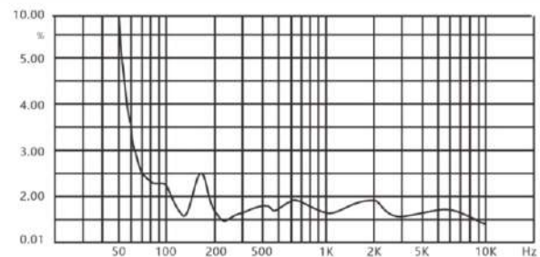
CNS8062 Distortion (THD < 5% 1W, 1m, 100Hz-10kHz)
