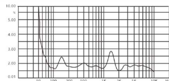
CNS8064 Distortion (THD < 5% 1W, 1m, 100Hz-10kHz)
