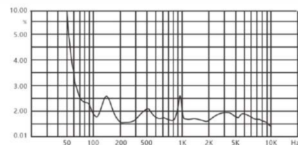
CNS8063 Distortion (THD < 5% 1W, 1m, 100Hz-10kHz)
