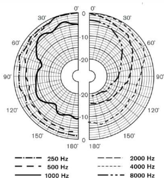
CNS8063 Horizontal Directivity Pattern
