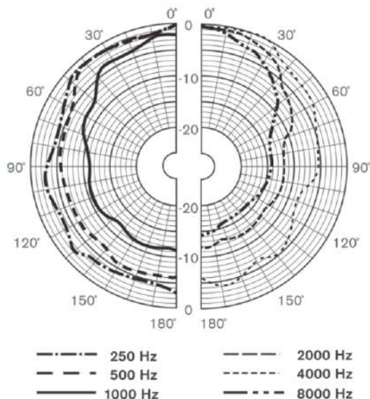
CNS8064 Vertical Directivity Pattern
