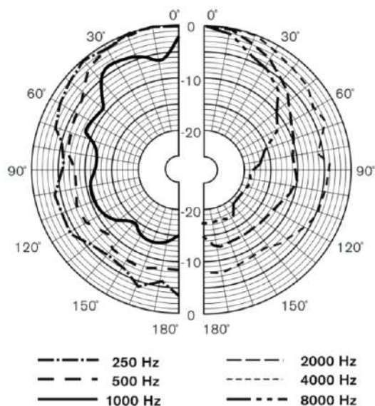
CNS8063 Vertical Directivity Pattern
