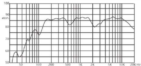
CNS8062 Frequency Response (dB SPL, 1W, 1m)
