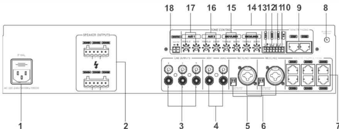
CNS5624MX Rear Panel
