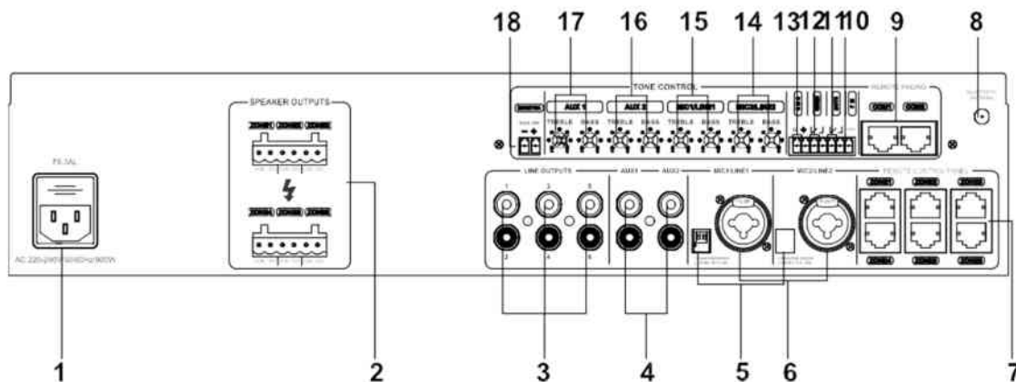
CNS5612MX Rear Panel
